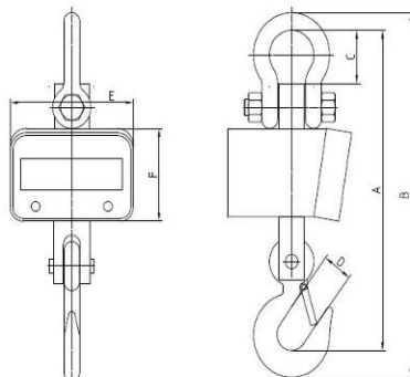
KPZ 406, 1 – 10 t
